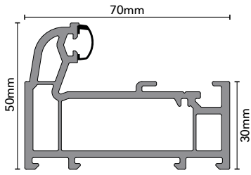
4F1 Slim Outer Frame
