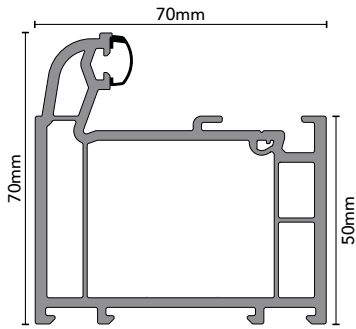
4F2 Large Outer Frame
