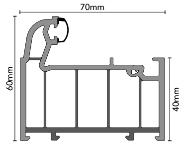
4F5 Multi-Chambered Outer Frame
